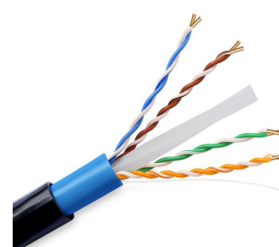
室外超六类非屏蔽阻水网线 Outdoor UTP Cat6
